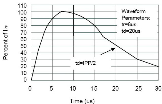
Pulse Waveform
