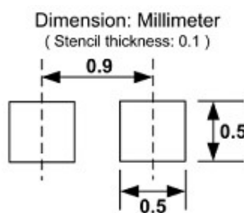
Soldering Footprint
