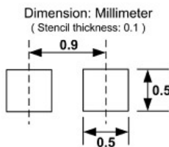
Soldering Footprint
