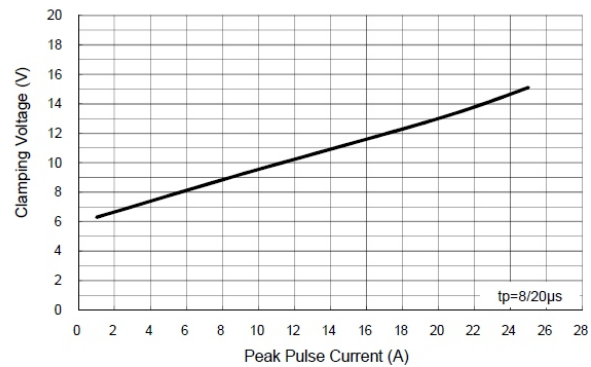
Fig 4 Peak Pulse Current vs Clamping Voltage
