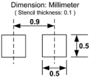
Soldering Footprint
