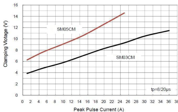
Fig 4 Clamping Voltage vs Peak Pulse Current
