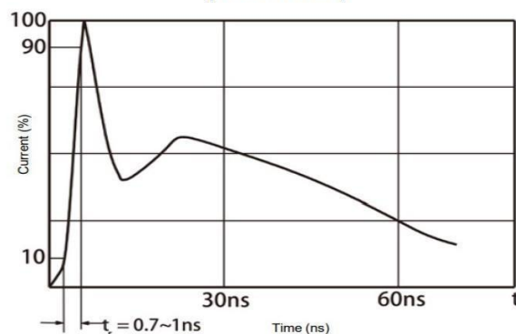
Fig 2 Contact Discharge Current Waveform per IEC 61000-4-2)
