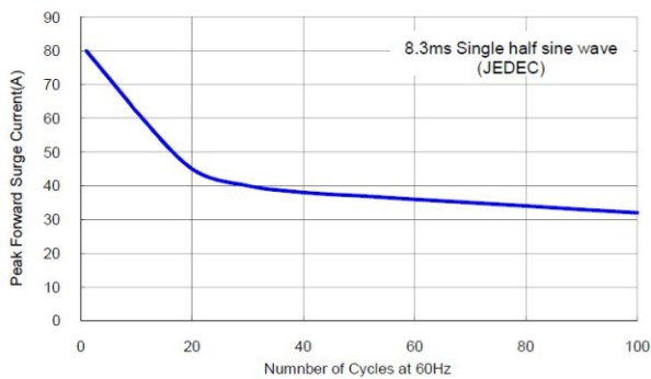
Fig 3 Max. Non-repetitive Forward Surge Current
