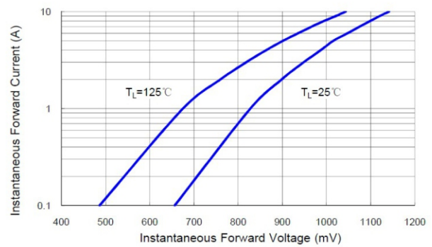
Fig 2 Typical Instantaneous Forward Characteristics
