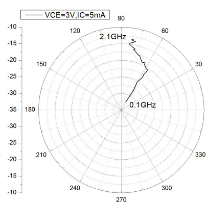
S_{12e} -FREQUENCY
