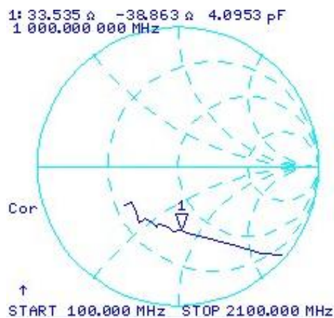
S_{22e} -FREQUENCY
