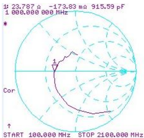
S_{11e} -FREQUENCY
